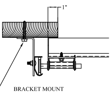
BRACKET MOUNT 5/16" x 1 5/8" LAG SCREW (1) PER JAMB BRACKET (1-1/2" EMBEDMENT MINIMUM) (TYP.)
